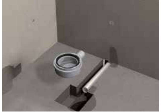
2. Fit the horizontal waste into position within the concrete floor.
